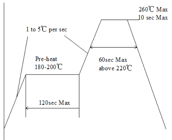
Recommended Reflow Soldering Condition (Lead-free solder)
