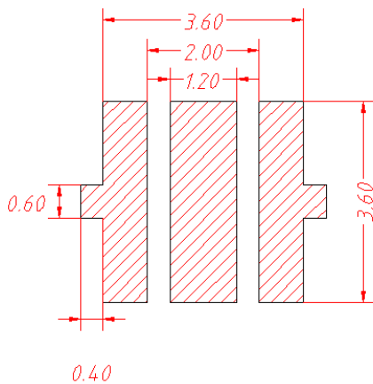
Recommended Soldering pad Layout (Unit: mm)
