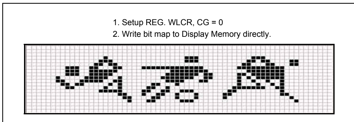
Figure 7-5: Graphics Mode
