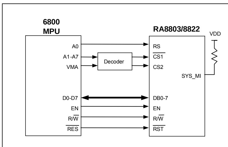
Figure 6-2: 6800 (8-Bit Only) MPU Interface
