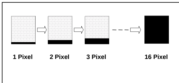
Figure 7-8: Cursor Height
