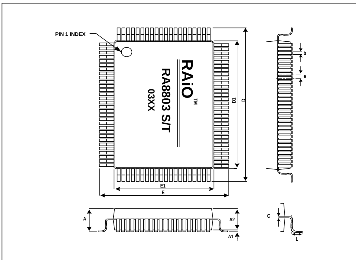
Figure 8-3 : PQFP-100Pin Mechanical
